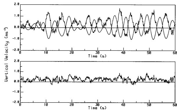
FIG. 5. The top panel shows a time series of the measured sonic vertical velocity (solid line) with the high-passed vertical velocity correction W_{hp}(t) . The bottom panel shows the true vertical velocity computed from Eq. (10).
